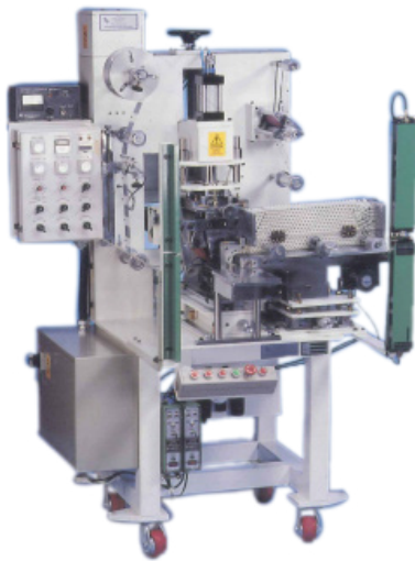
R-070 Automatic Feed System This machine has a production rate of 25 Pens each per minute.
